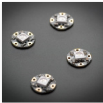
Adafruit Flora RGB Smart Neo Pixel version 2 - Pack of 4
